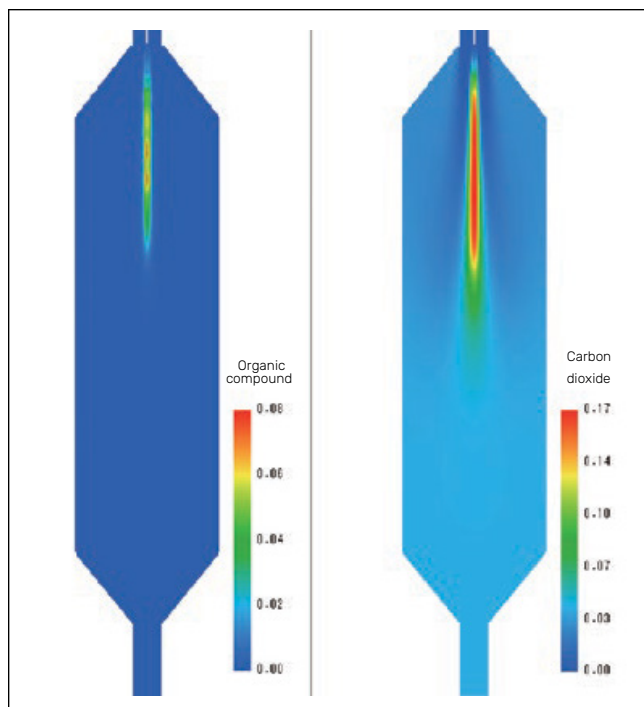
Figure 5: Mass fraction distribution of combustion gases (8 sec.), organic compound (left), carbon dioxide (right)
