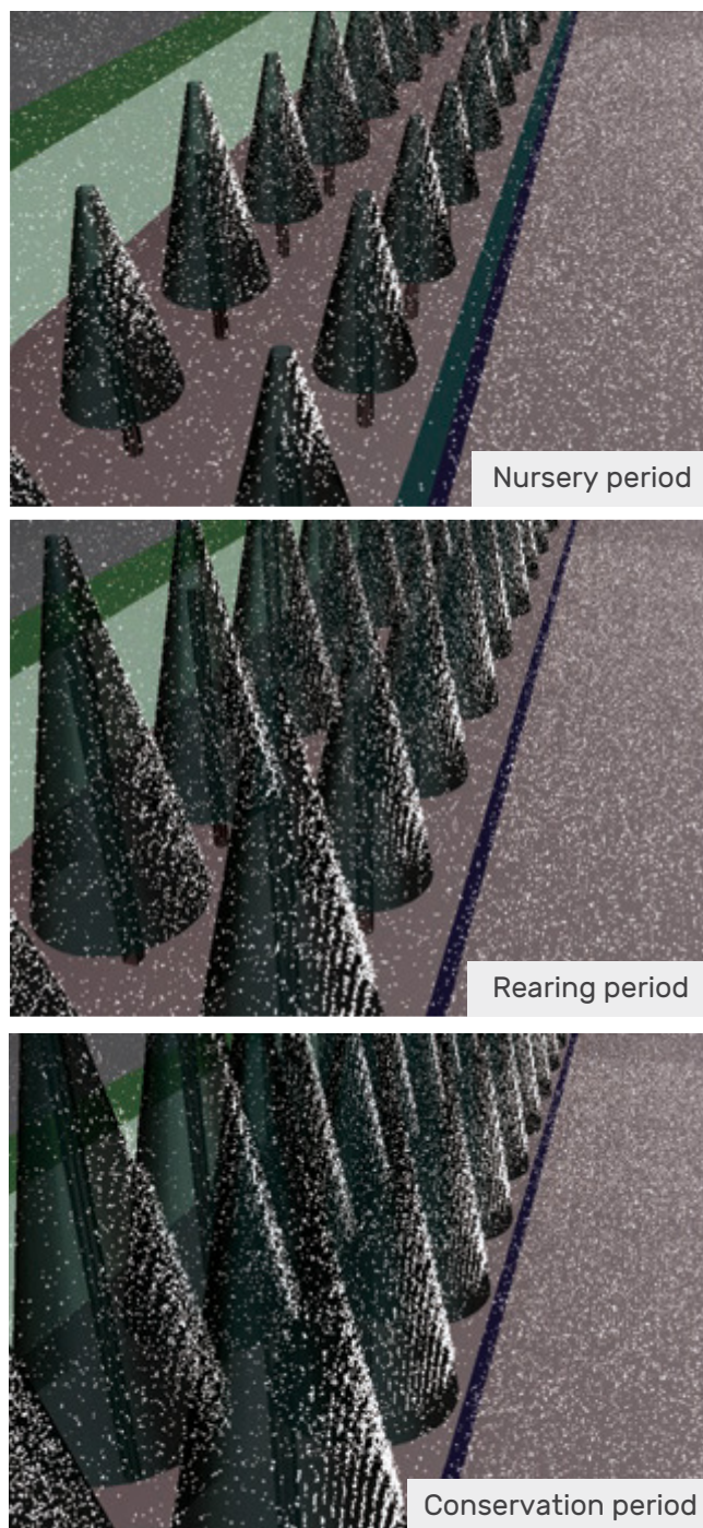
Figure 6: Snow particle behavior
