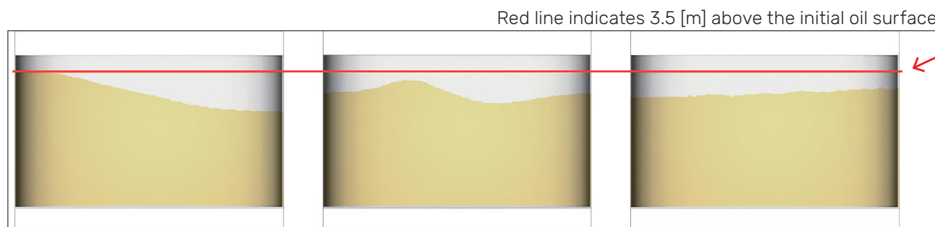
Figure 2: The maximum oil surface height. Left: 5 sec. period ( t=13 [sec.]), middle: 4 sec. period ( t=15 [sec.]), right: 2 sec. period ( t=17 [sec.])
