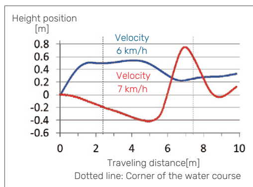
Figure 6: Relation between the height position of the vehicle and the traveling distance
