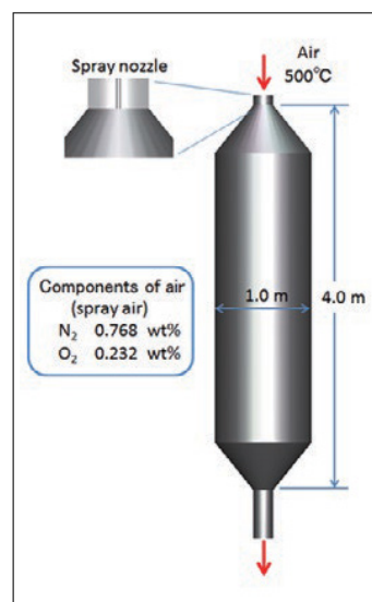
Figure 3: Combustion chamber
