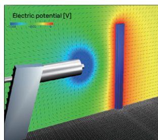
Figure 3: Electric potential distribution
