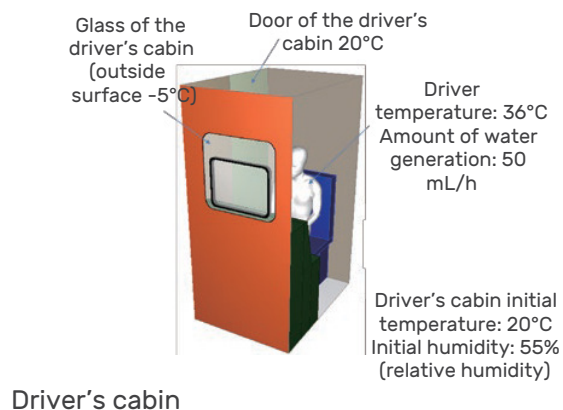
Figure 2: Railroad car
