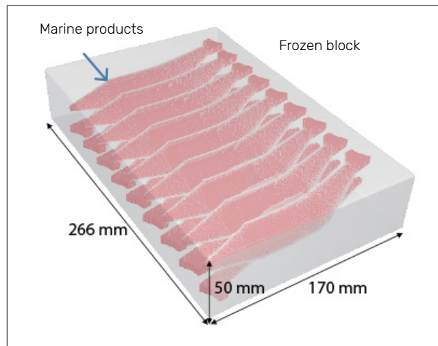
Figure 3: Frozen block
