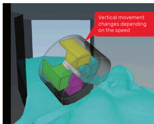
Figure 5: 3 seconds after the ride vehicle went in motion (speed 7 km/h)
