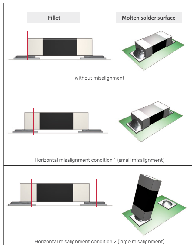
Figure 3: Molten solder analysis results (without misalignment [top], horizontal misalignment condition 1 [middle], horizontal misalignment condition 2 [bottom])
