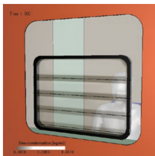
Figure 3: Temperature distribution of glass of the driver's cabin (above), dew condensation distribution (below)
