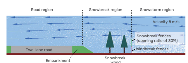
Figure 1: Snowbreak trees along the road
