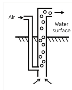
Figure 1: Airlift pump
