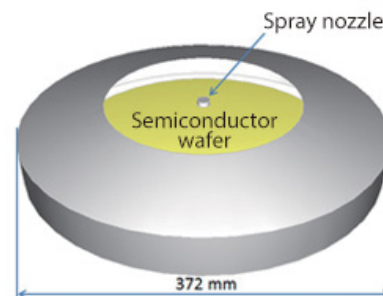
Figure 2: Single-wafer cleaner
