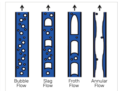
Figure 2: Types of two-phase flow
