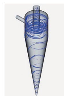
Figure 6: Streamlines
