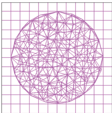
Figure 1: Overset mesh
