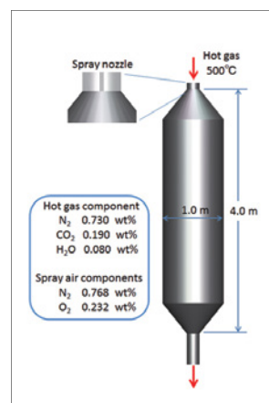
Figure 1: Spray air nozzle
