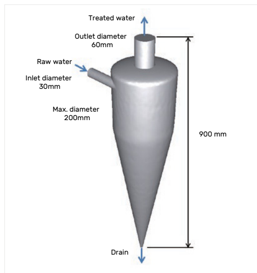
Figure 4: Sand separator
