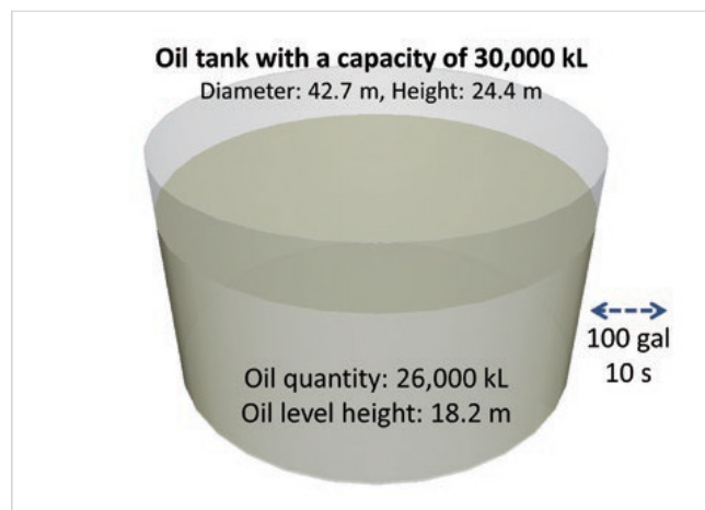
Figure 1: Oil tank with a capacity of 30,000 [kL]
