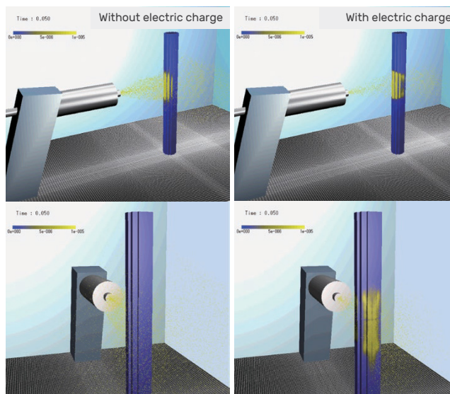
Figure 4: Analysis result (0.05 sec.) Paint distribution in front (top), paint distribution in back (bottom)
