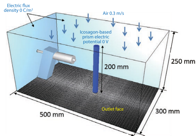
Figure 1: Coating booth
