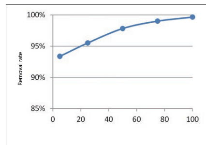
Figure 7: Variation of the sand removal rate depending on the particle diameter
