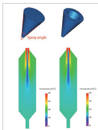
Figure 2: Temperature distribution (7 sec.) Full-cone (left), hollow-cone (right)
